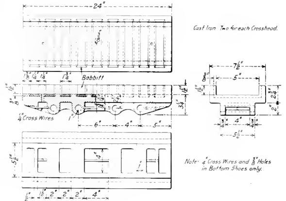
Type of Shoe for Which the Jig is Used
